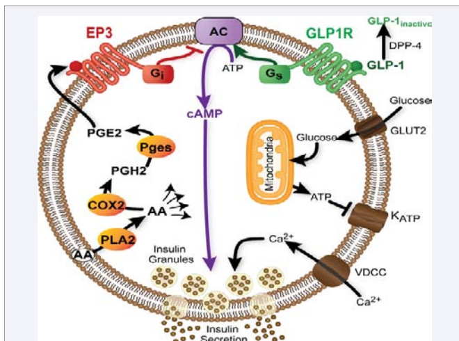
Figure 1 PGE2 signaling through EP3 negatively regulates beta-cell function. AA is cleaved from membrane phospholipids by phospholipase A2 (PLA2). PGE2 is generated by two sequential enzymatic steps: cyclooxygenase 2 (COX2)-mediated generation of PGH2, followed by prostaglandin E synthase (Pges)-mediated conversion to PGE2. PGE2 can activate the EP3 receptor on the beta-cell to block cAMP production, interfering with cAMP-mediated signaling through the GLP-1 receptor.
