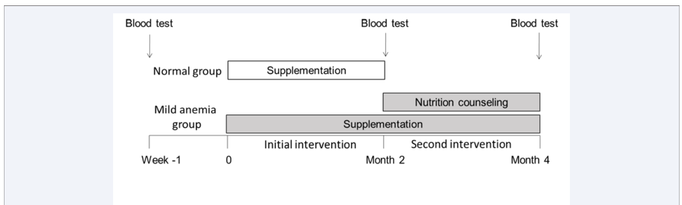
Figure 1 Study design.
