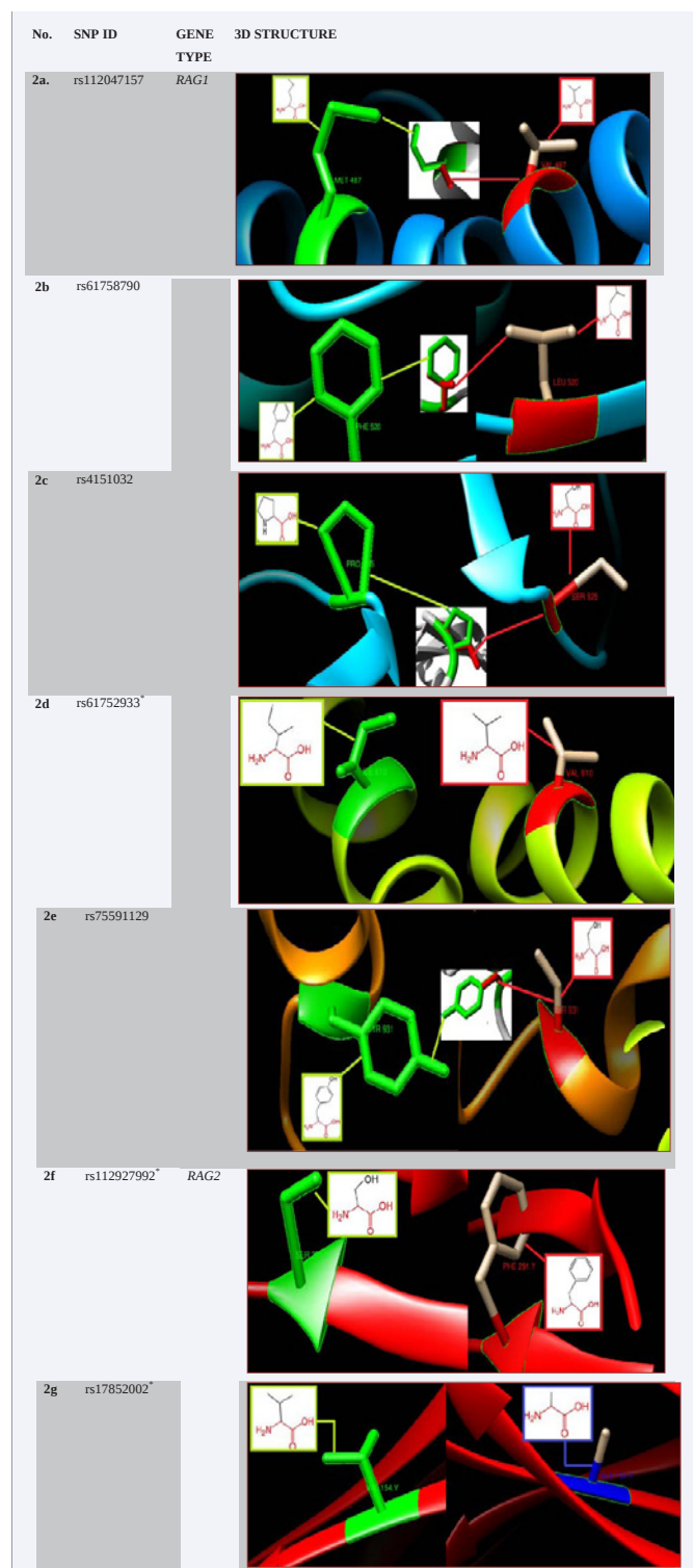
Figure 2 3D model by Chimera and Project HOPE for RAG1 and RAG2 proteins.
