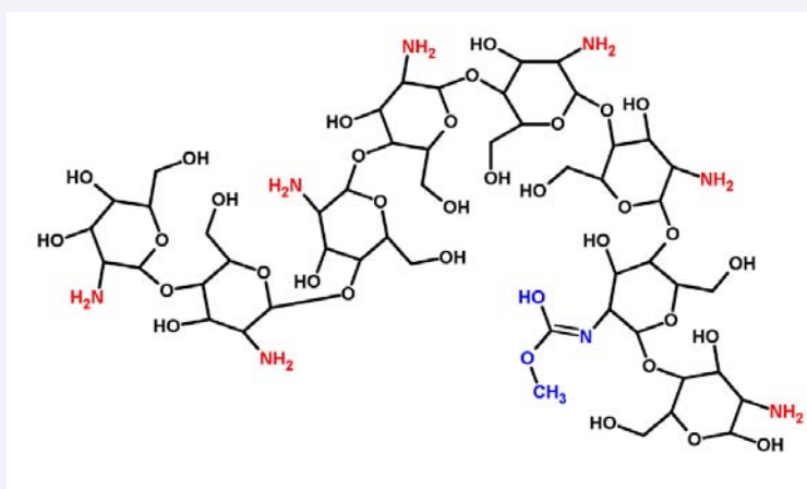
Figure 1 Chitosan structure. The interaction between reactive radicals allows the formation of a complex construction in the polymer matrix. Glucosamine amino group (red) and acetamido groups (blue) from n-acetyl glucosamine are highlighted.
