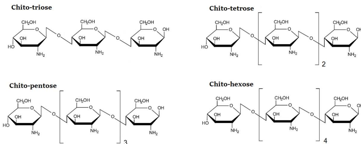
Figure 2 Some chito-oligosaccharides structure. The main component of CHOS is glucosamine connected by \beta (1-4) glycosidic bonds. CHOS usually has a higher deacetylation degree due to their conformation.
